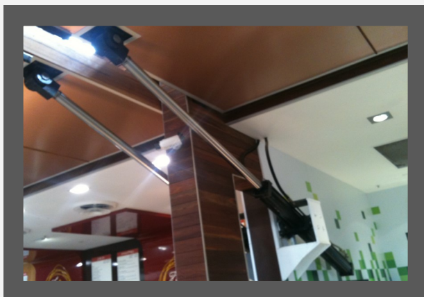
Trunnion mounted cylinders lift the doors
